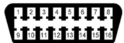
FRONT VIEW OF OBD CONNECTOR
