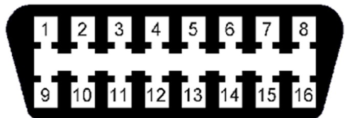
FRONT VIEW OBD CONNECTOR
